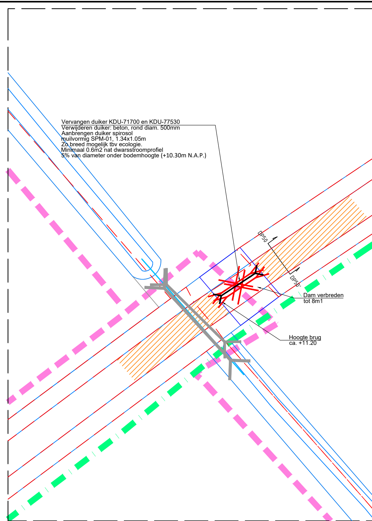
Detail 6.2 Schaal: 1:200
