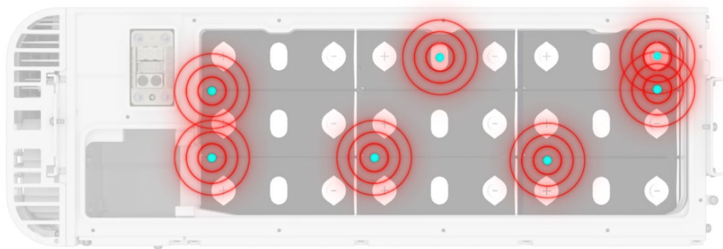
Figure 9: Seven temperature sensors for nine battery cells – © Sigenergy (2024)
