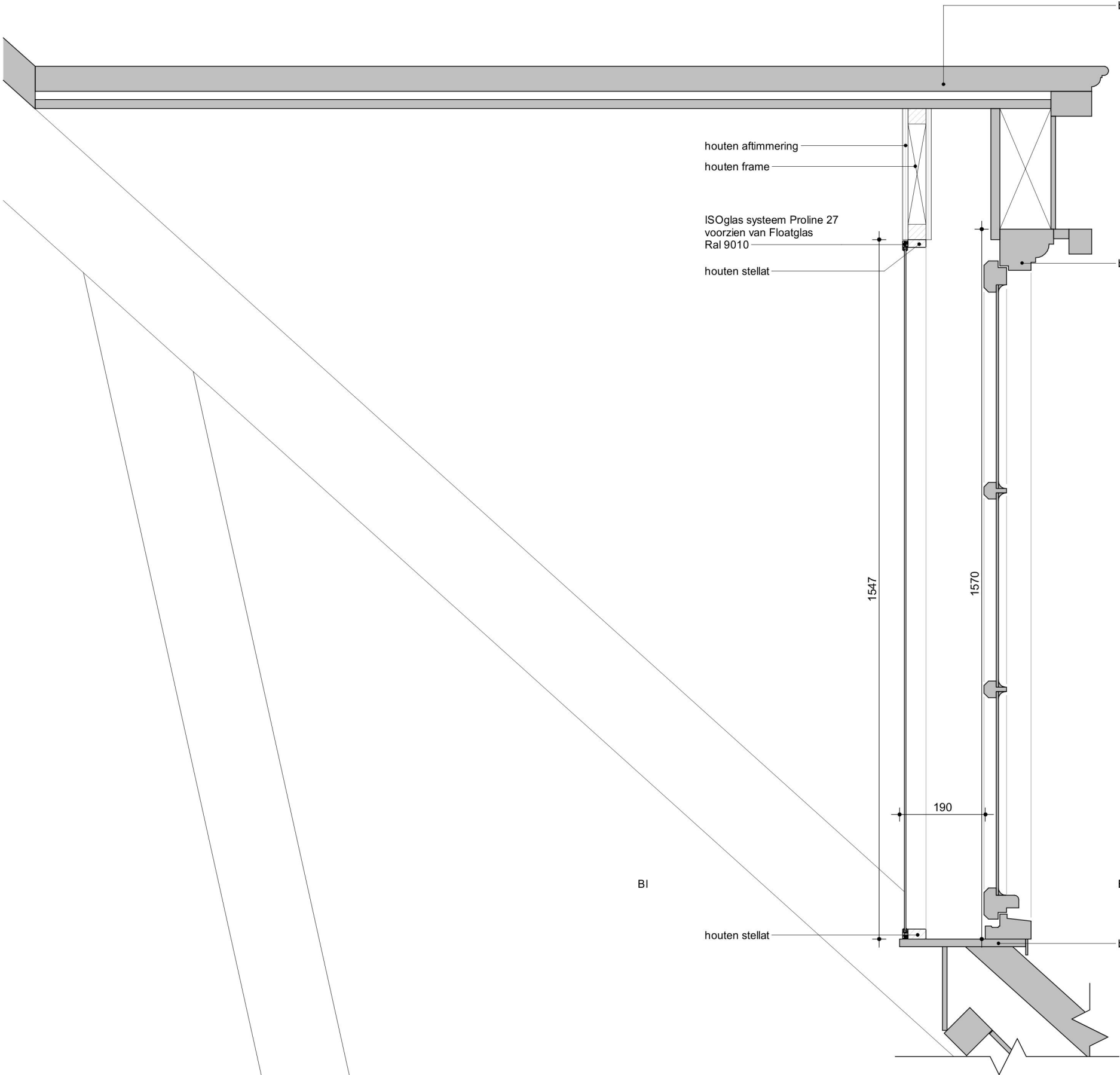
Merk 5A.05 - Nieuw detail N09-V
