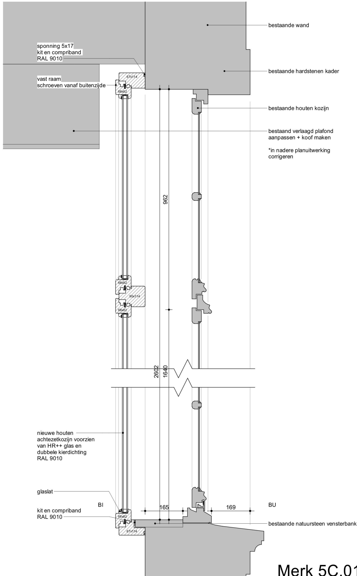
Merk 5C.01 - Nieuw detail N26-H
