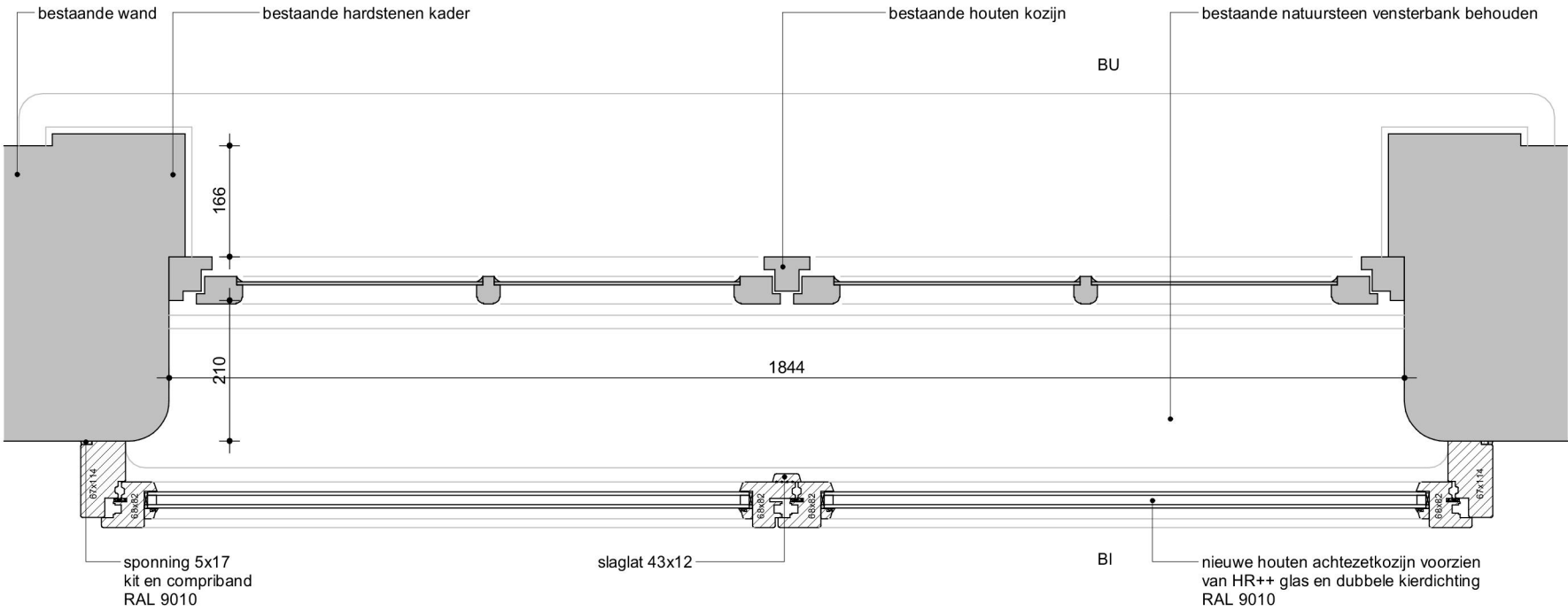
Merk 5C.01 - Nieuw detail N26-H
