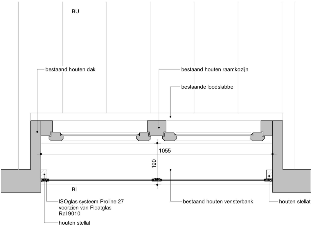
Merk 5A.05 - Nieuw detail N10-H
