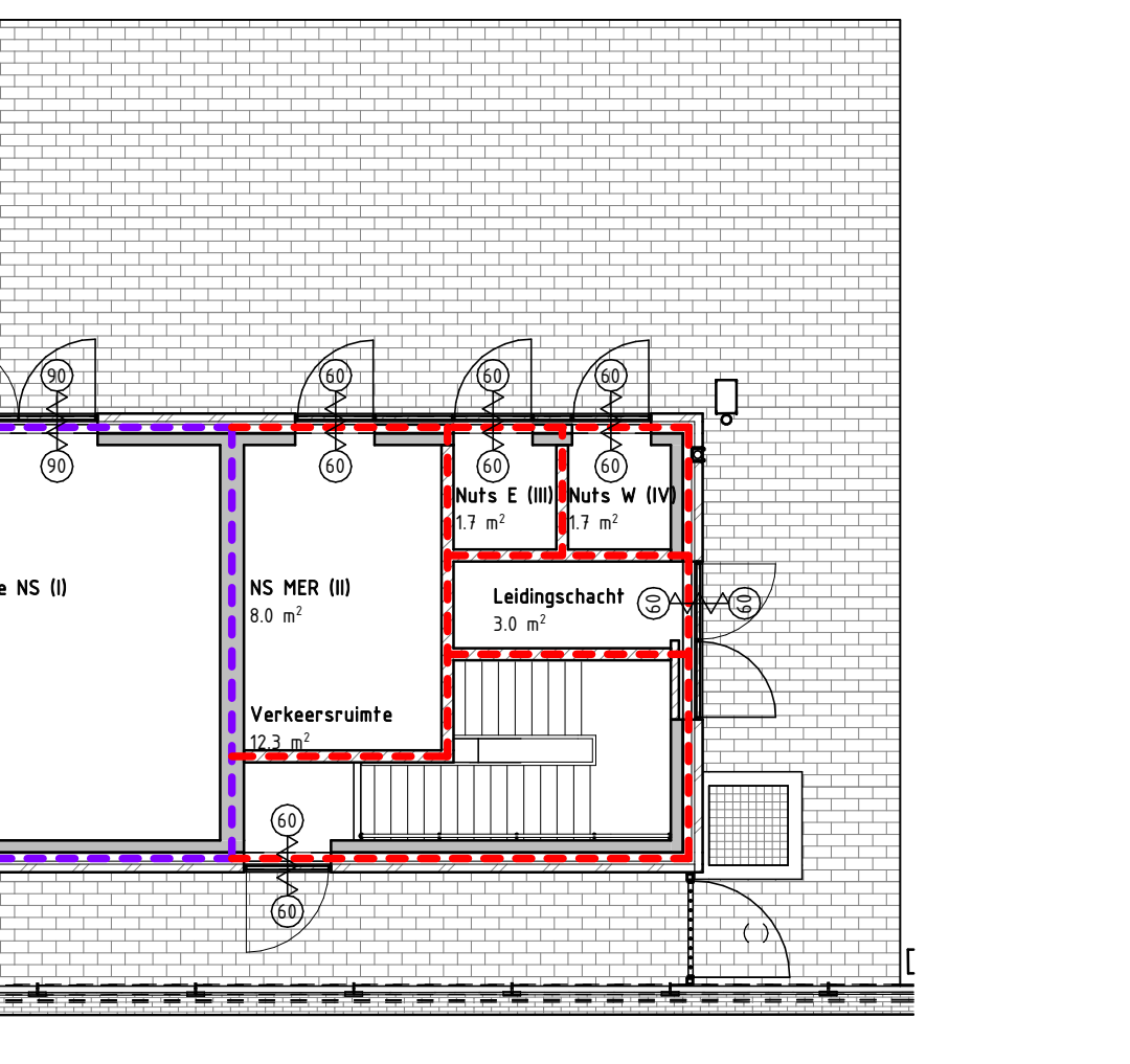
Begane grond TG Brandwerendheid
