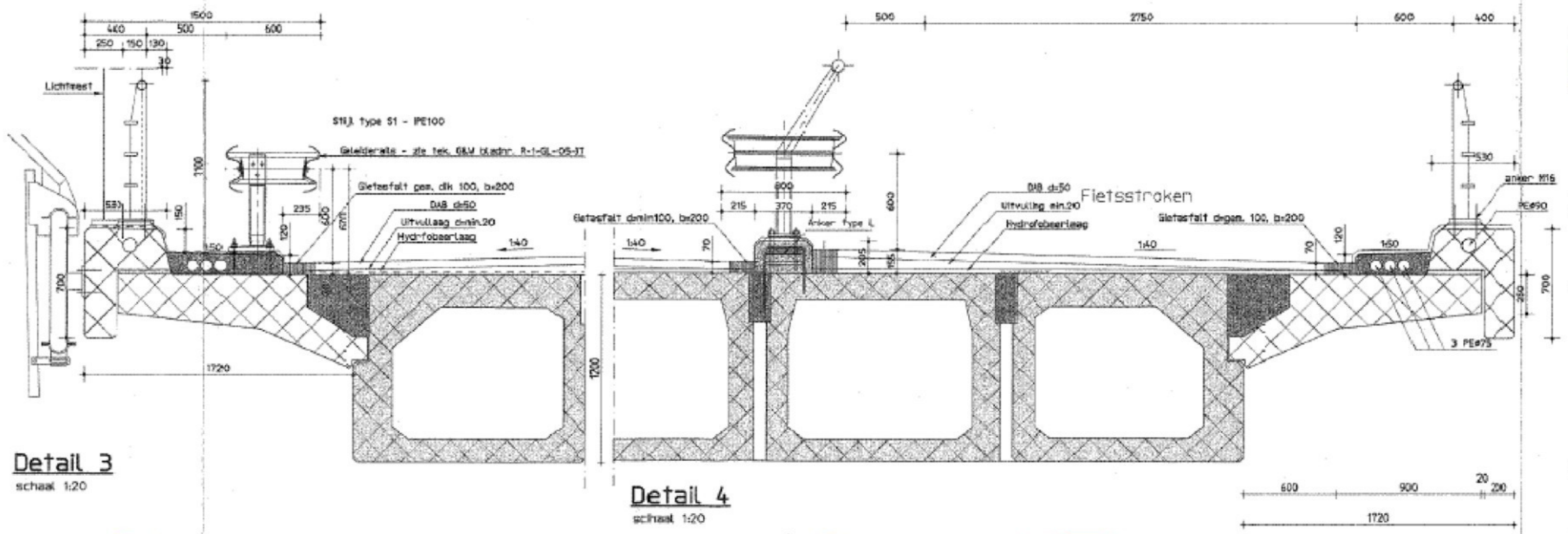
Detail wegviaduct A16
