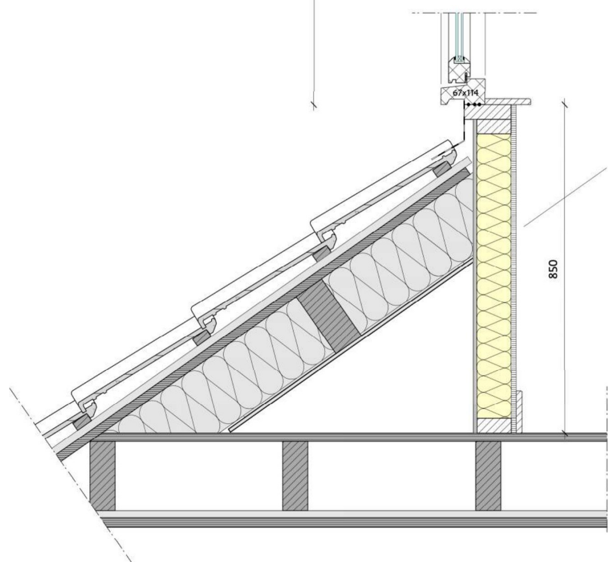
Detail 3
