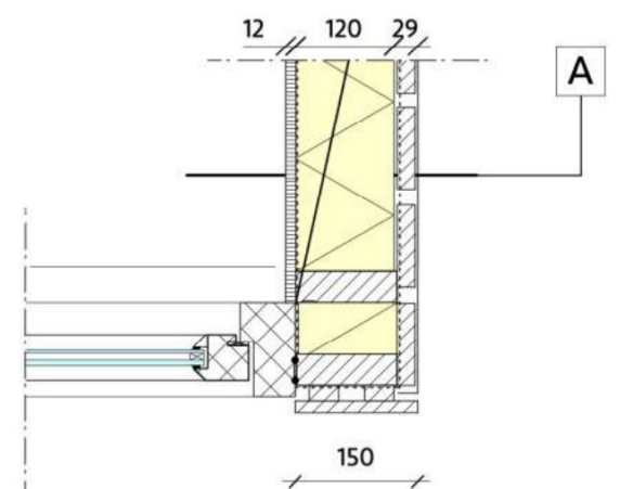
Detail 4
