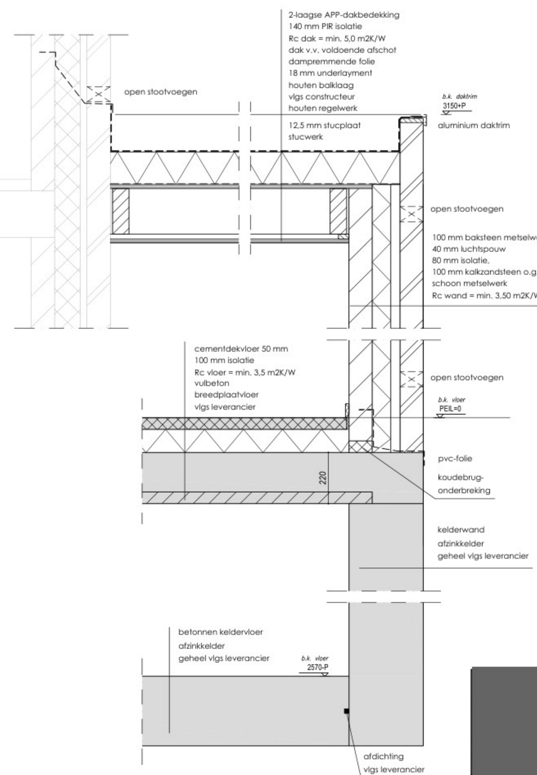
PRINCIPE-DETAILS
