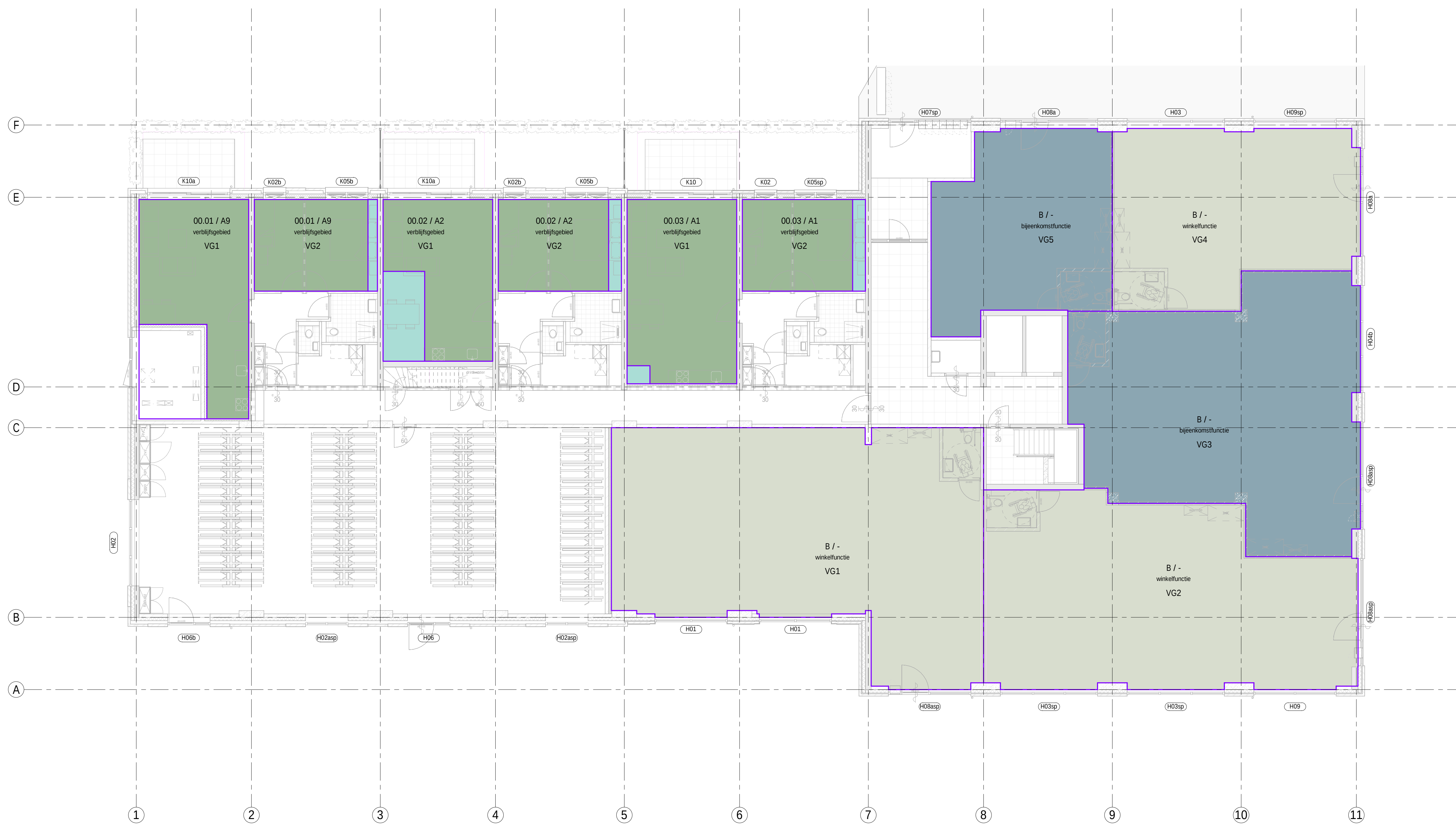
00 begane grond
