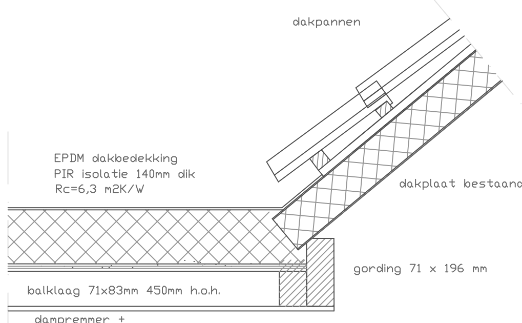
DETAIL -3-
