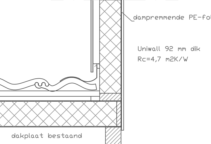
DETAIL -4-
