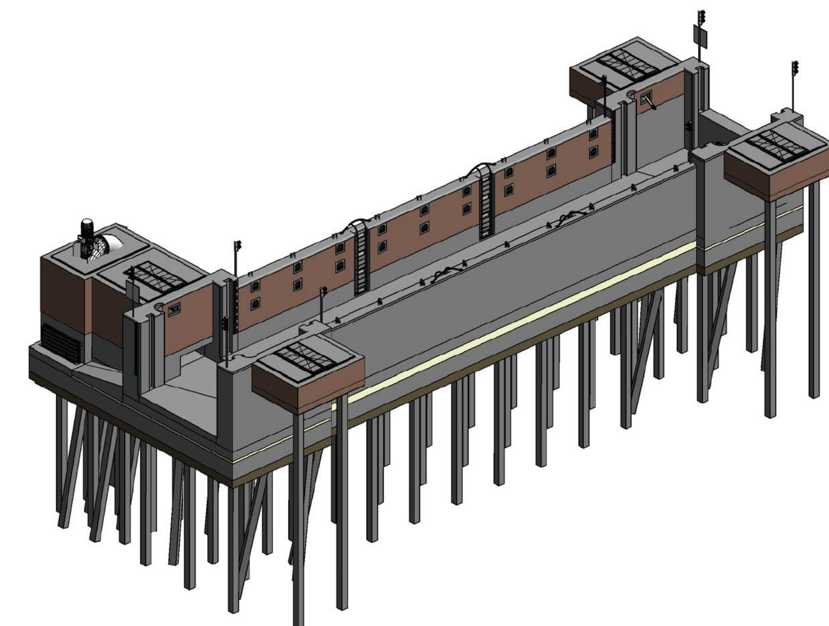
3D VIEW SLUIS
