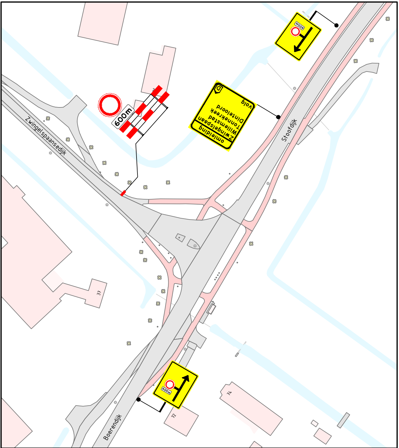
DETAIL 3 1:1000
