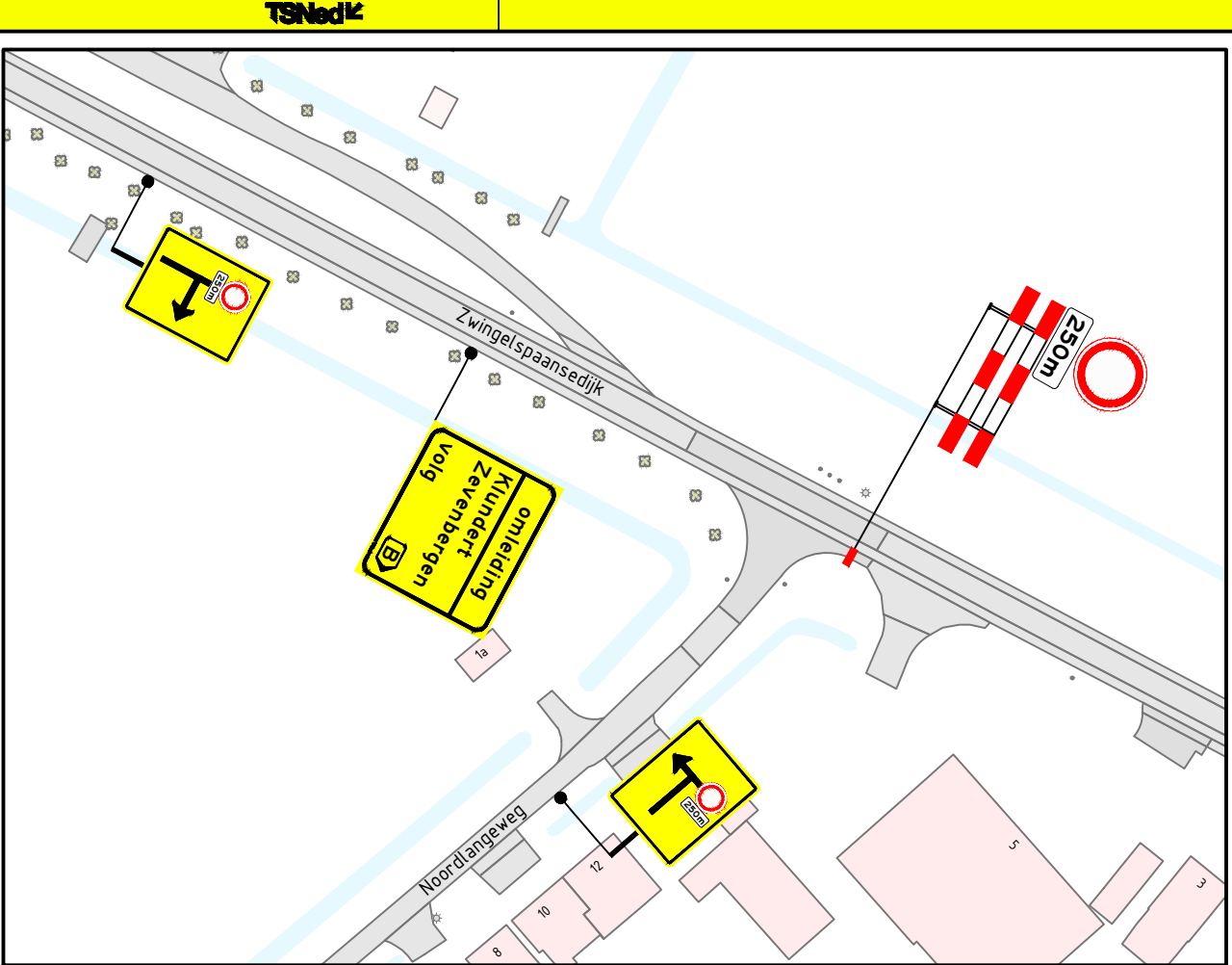
DETAIL 1 1:1000
