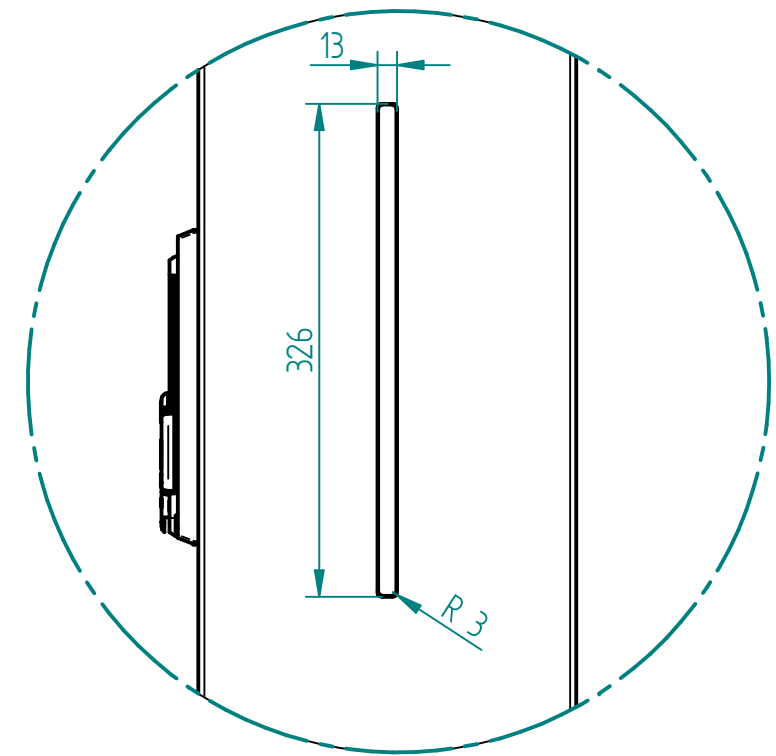
DETAIL D
