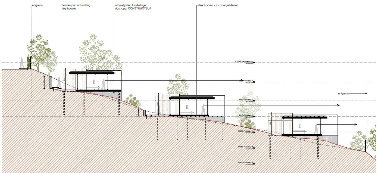
afb 8 - Doorsnede dormaetini's in de helling
