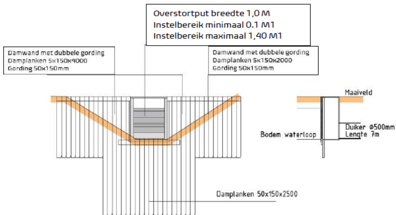
Lobstuw principe detail
