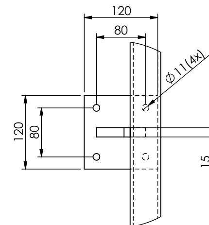
DETAIL B SCALE 1 : 6
