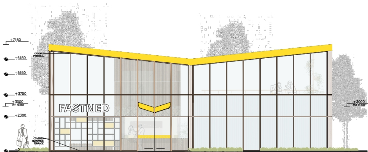
FRONT ELEVATION 1:150
