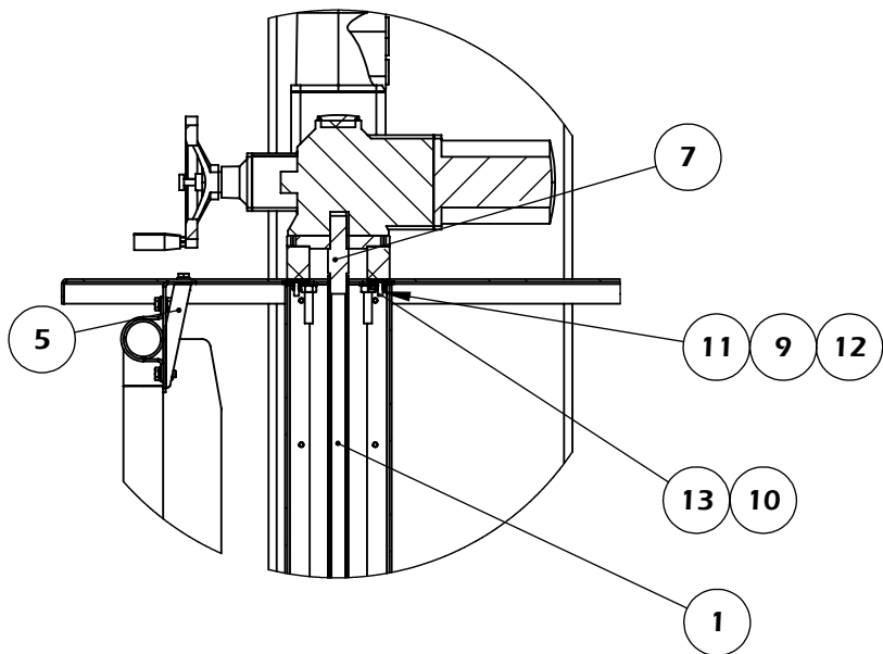
DETAIL F SCALE 1 : 10
