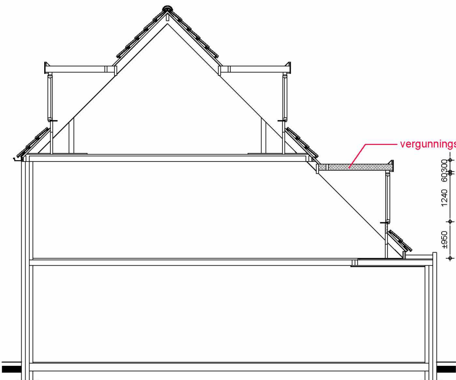
= Doorsnede nieuw =
