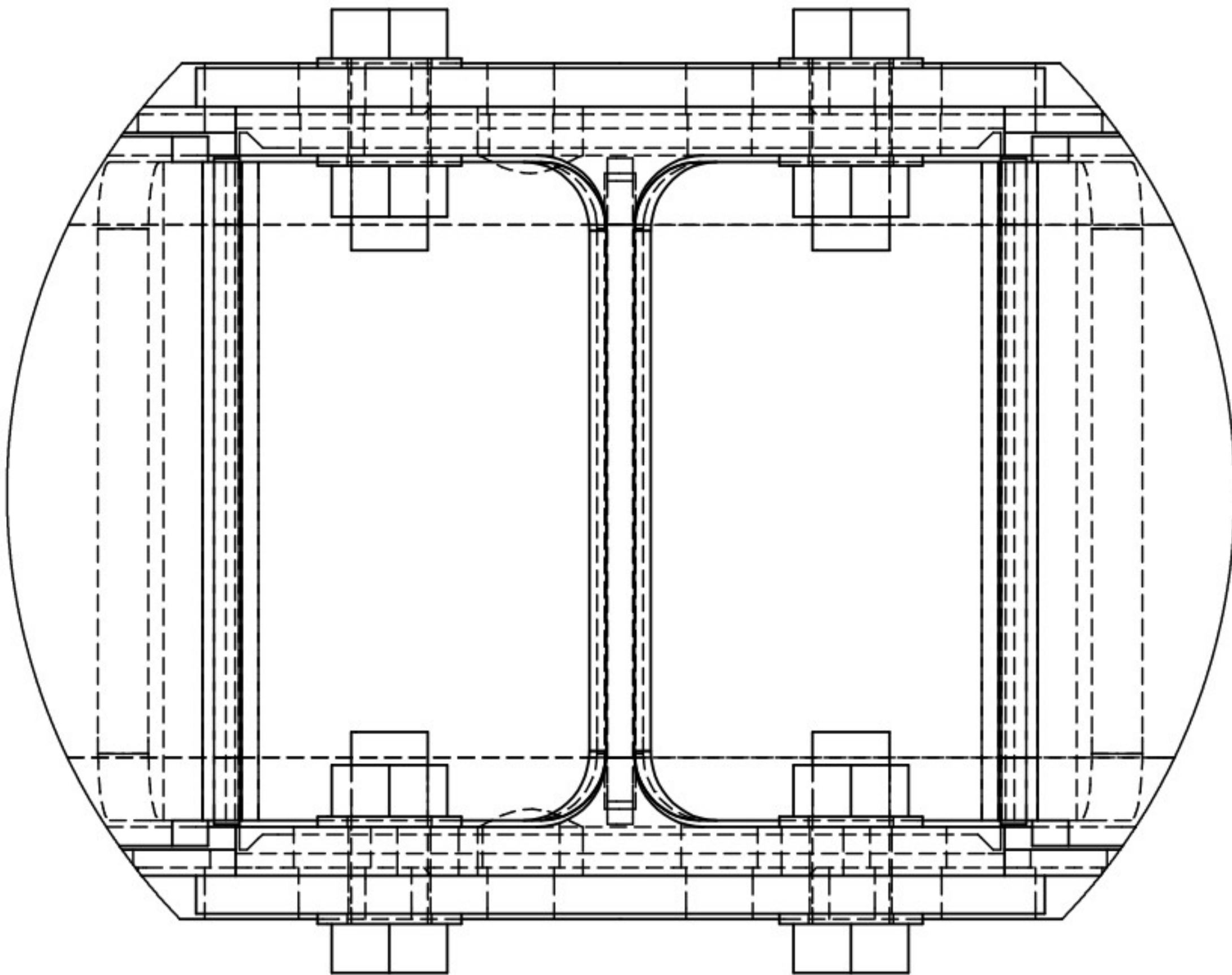
DETAIL C SCALE 1 : 5
