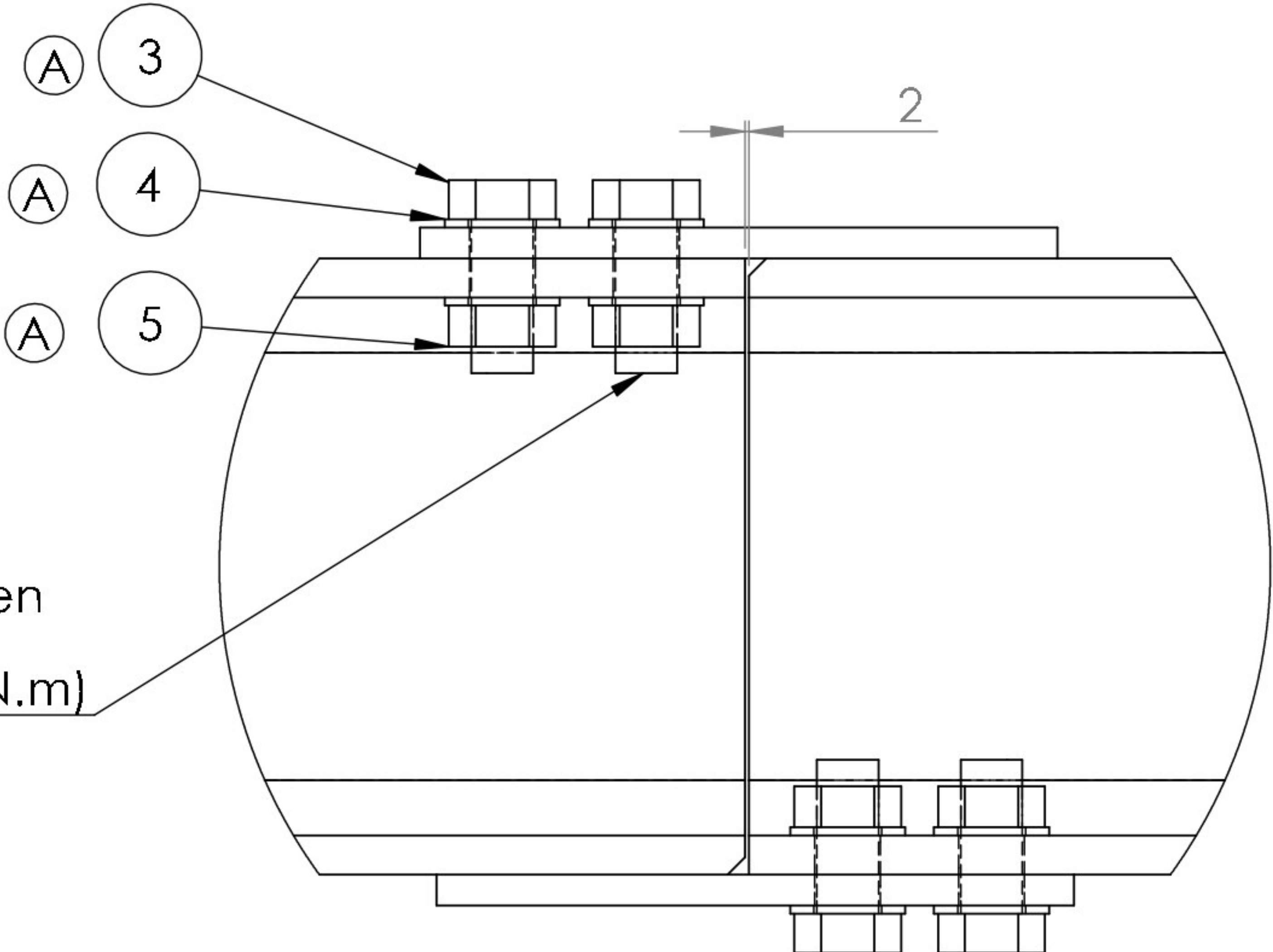
DETAIL D SCALE 1 : 5
