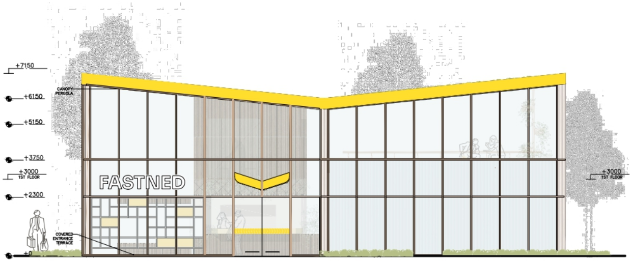
FRONT ELEVATION 1:150
