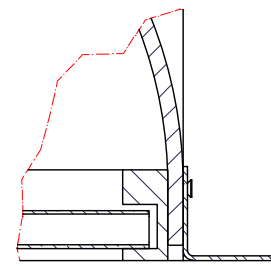
Detail C (1 : 5)
