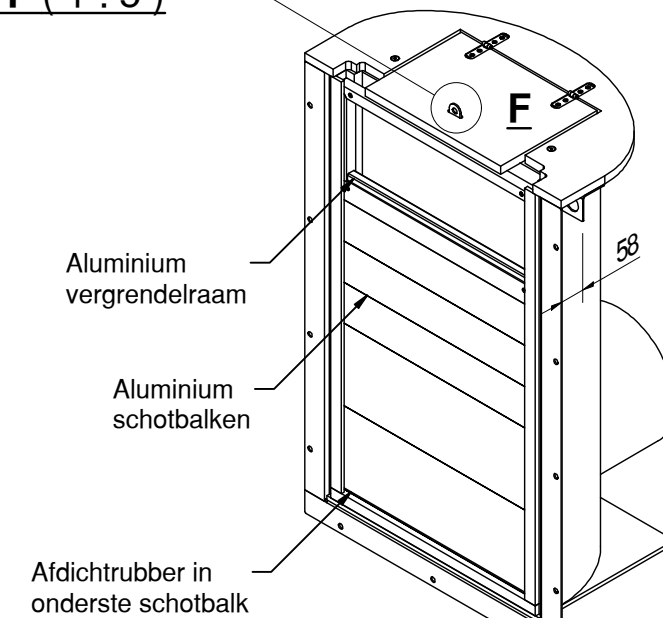
Detail F (1 : 5)
