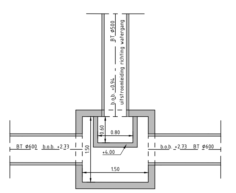
DETAIL 1: OVERSTORTPUT SCHAAL 150
