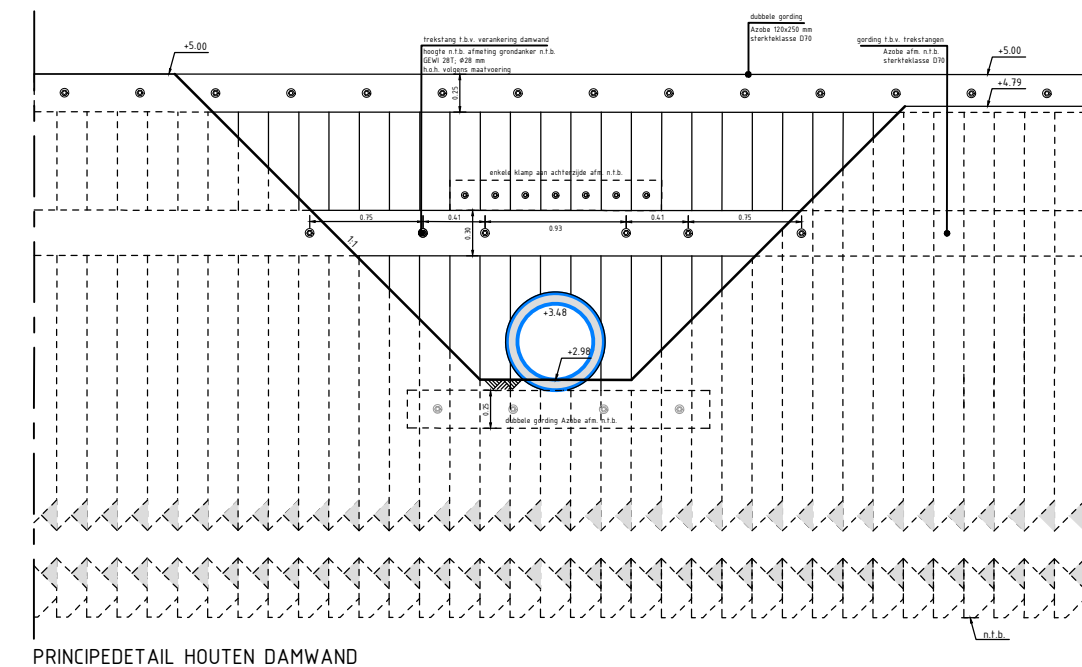
PRINCIPEDETAIL HOUTEN DAMWAND
