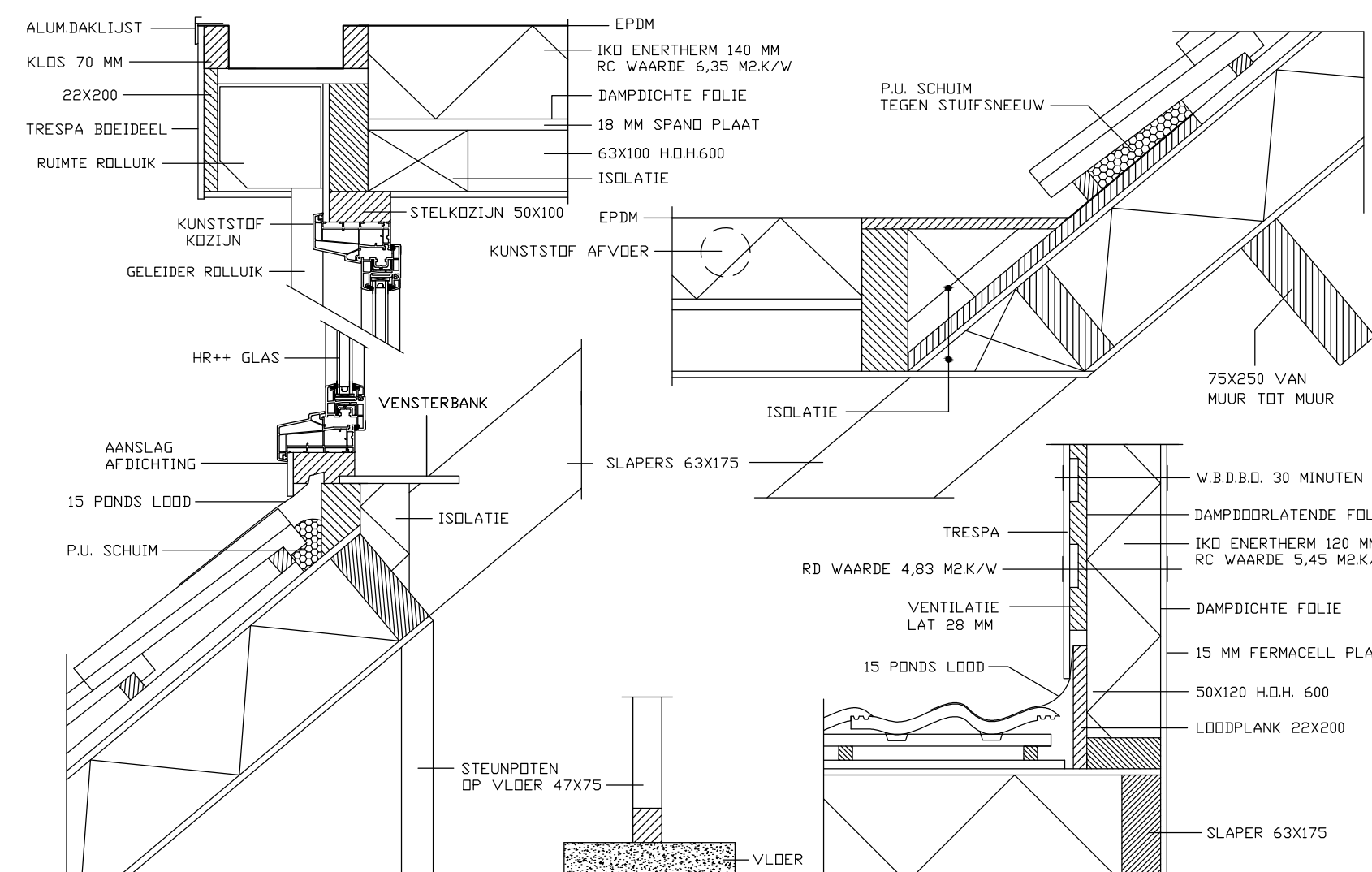
DETAIL SCHAAAL 1:10
