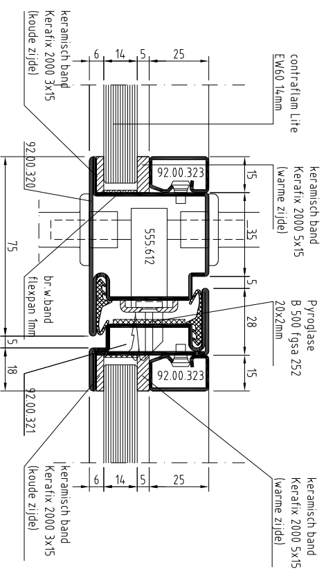
detail H2
