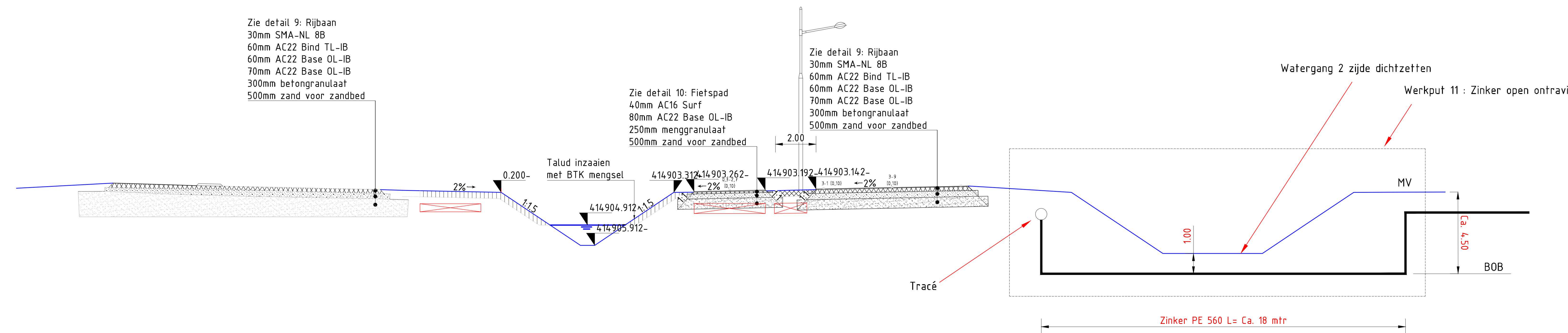
Metreering 6.754 8.502 10.000 11.511 24.675 28.561 30.000 30.624 34.524 38.457 40.017 43.282 46.124 50.000 52.896 54.372 58.697 60.000 61.133 63.197 68.097 72.597 74.899 77.504 Hoogte 0.024 0.117 0.205 0.258 -0.059 -0.147 -0.184 -0.200 -2.800 -0.645 -0.156 -0.087 -0.030 0.048 0.105 0.073 -0.200 -1.069 -1.824 -3.200 -3.200 -0.200 -0.191 -0.180
