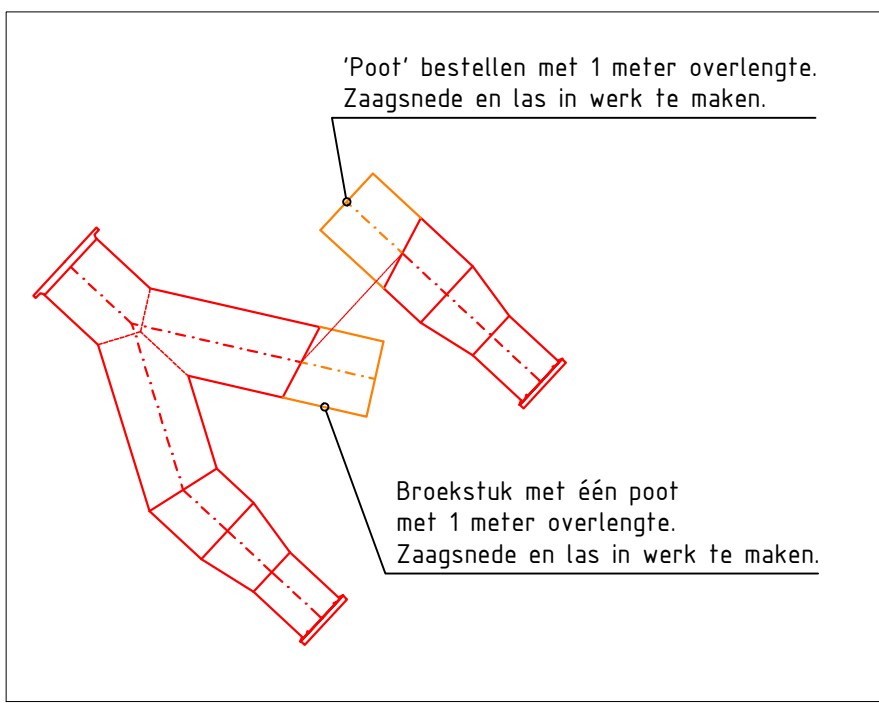
Detail B
