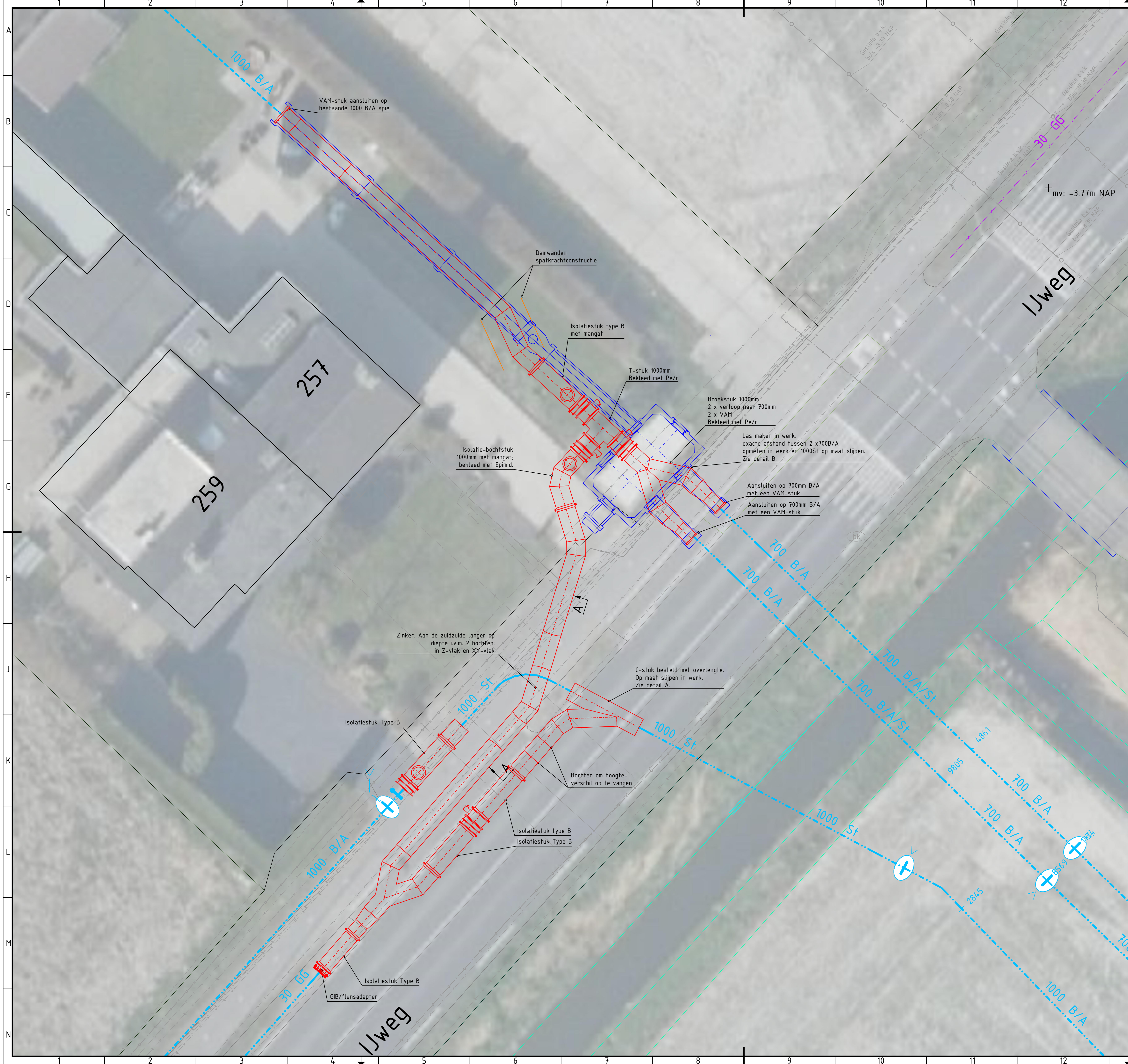
Detail A
