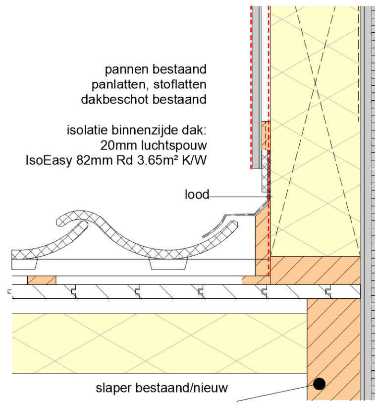
Detail 4
