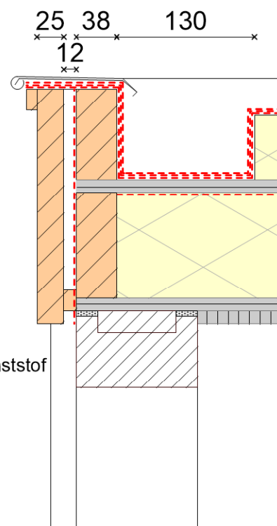
Detail 3
