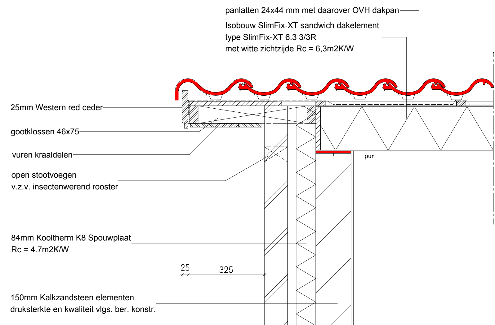
Detail 2 overstekdetail.
