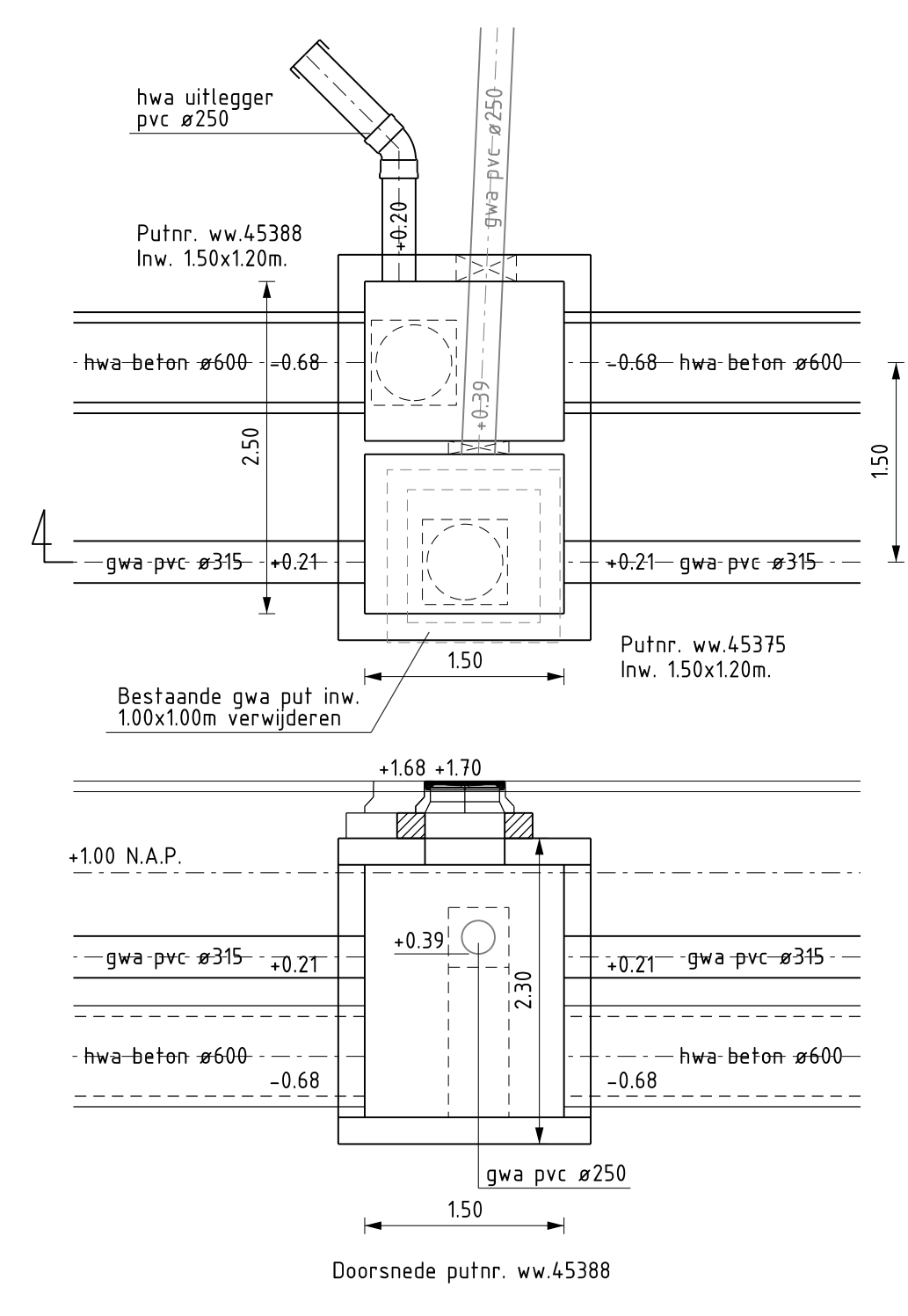
Detail D 150 Putnr. ww.45388 / ww.45375
