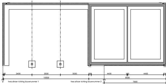
fundering / riolering
