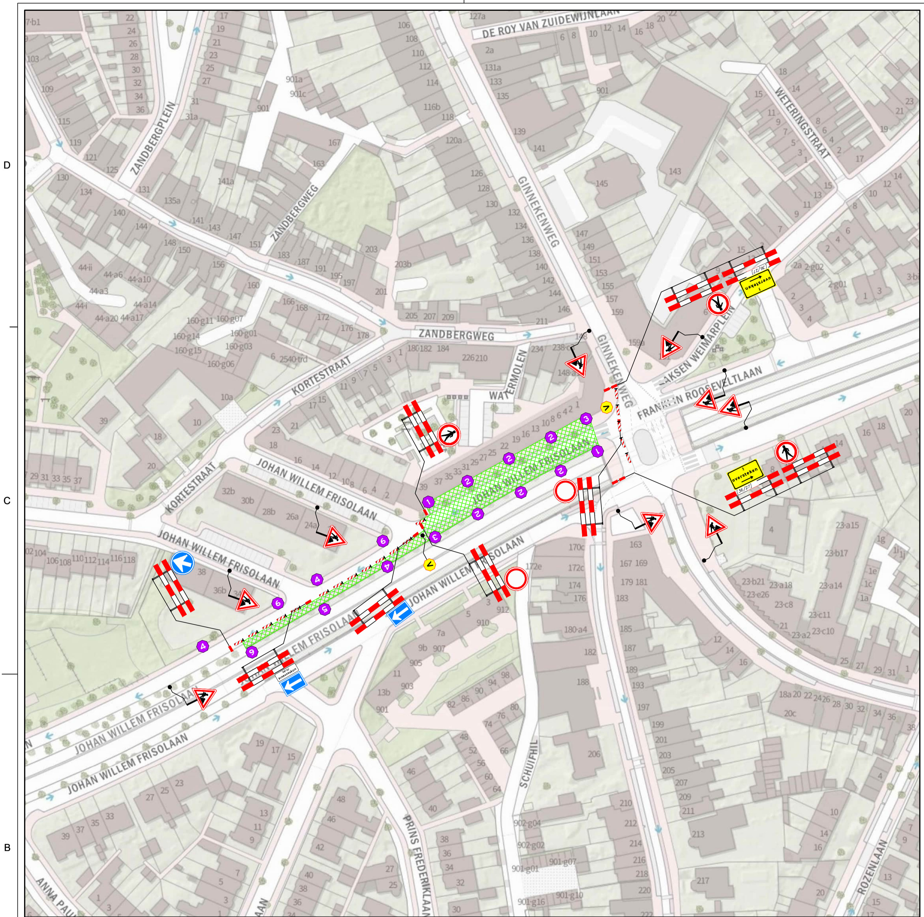
DETAIL A
