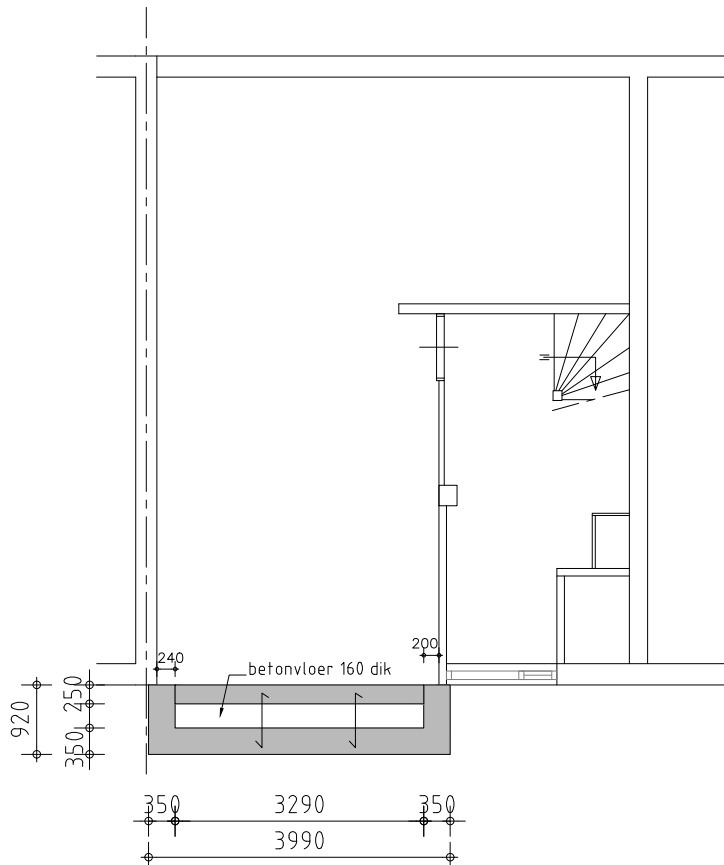
fundering
