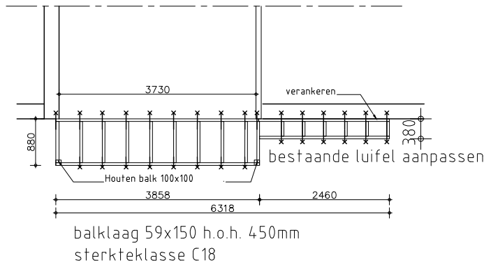
houten balklaag
