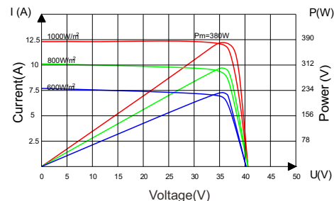
Current-Voltage&Power-Voltage Curve(380W)
