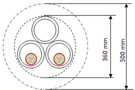
Principeprofiel boring
