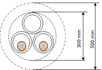
Principeprofiel boring
