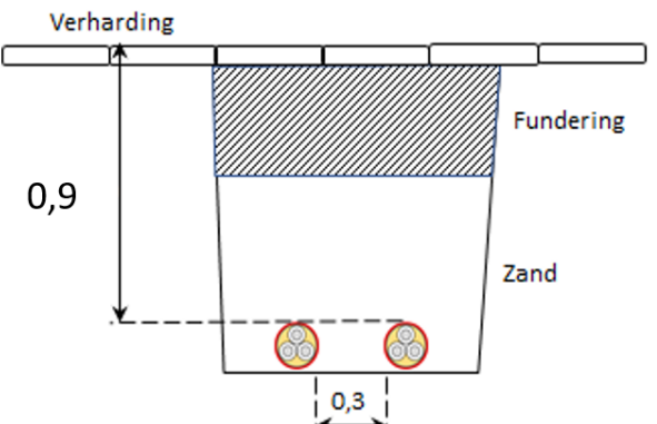
Principeprofiel open ontgraving
