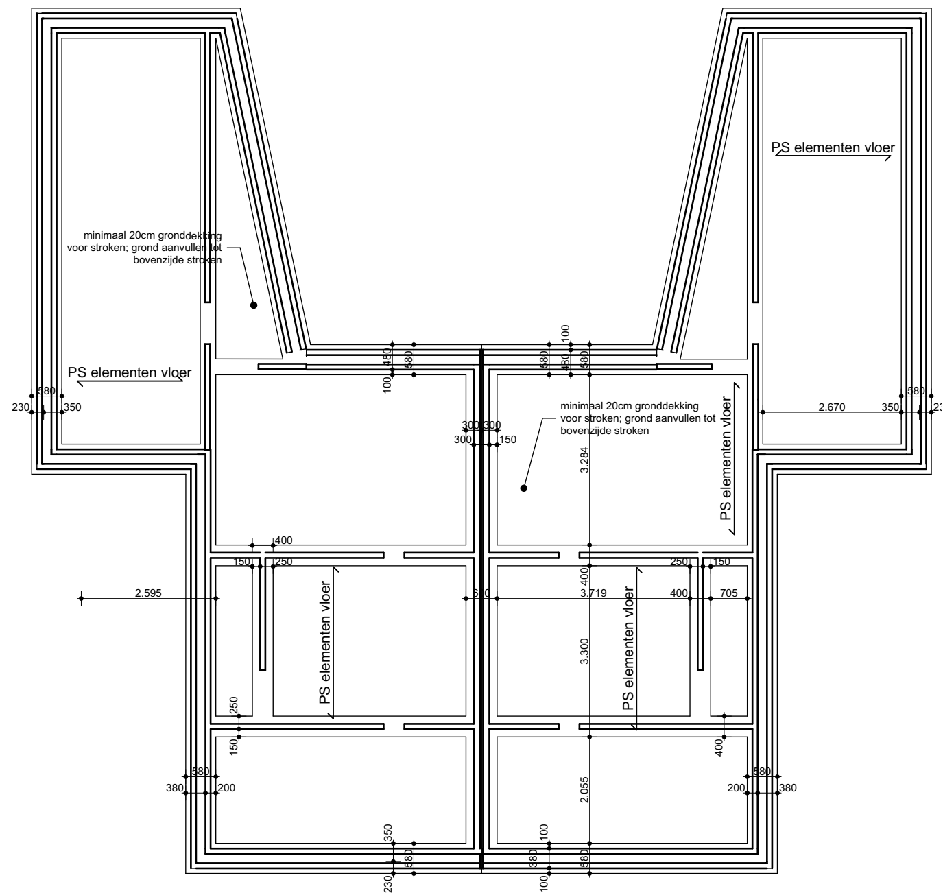
-1. Fundering/Begane grond 1:100
