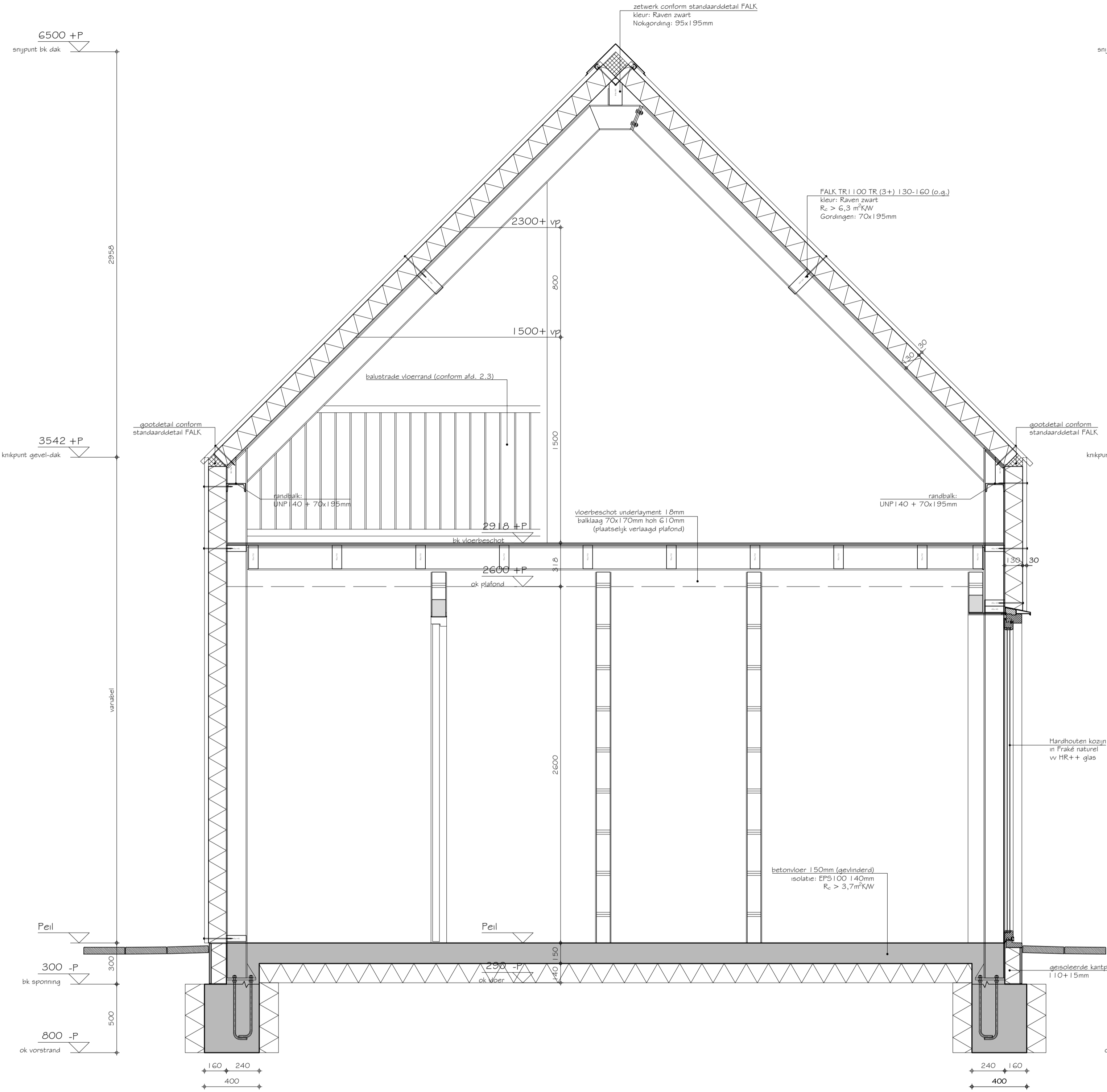
DOORSNED E C-C
