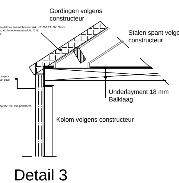
Detail 3
