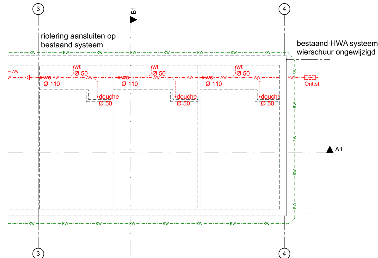
Riolering
