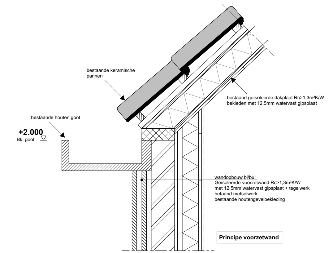
Detail 3
