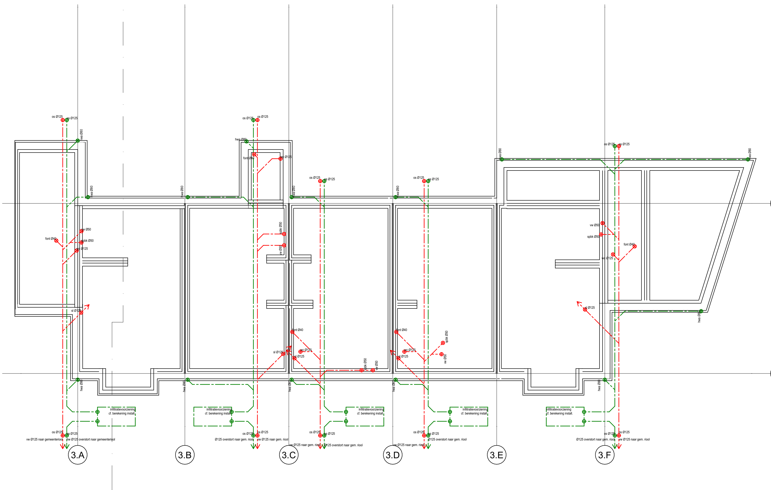
-1 fundering 1:100
