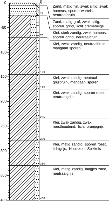
Boring A04
