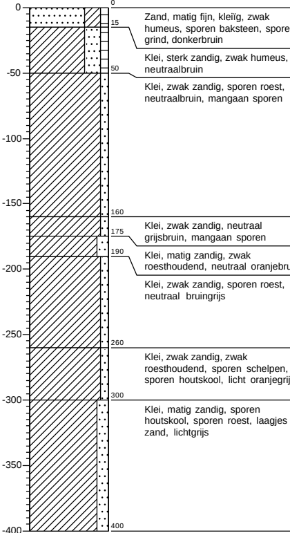
Boring A06
