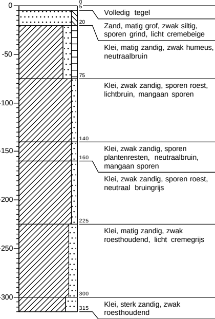
Boring A10
