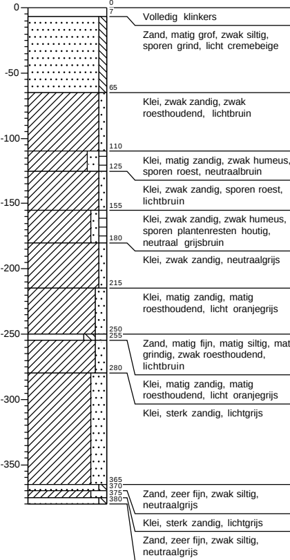
Boring A05
