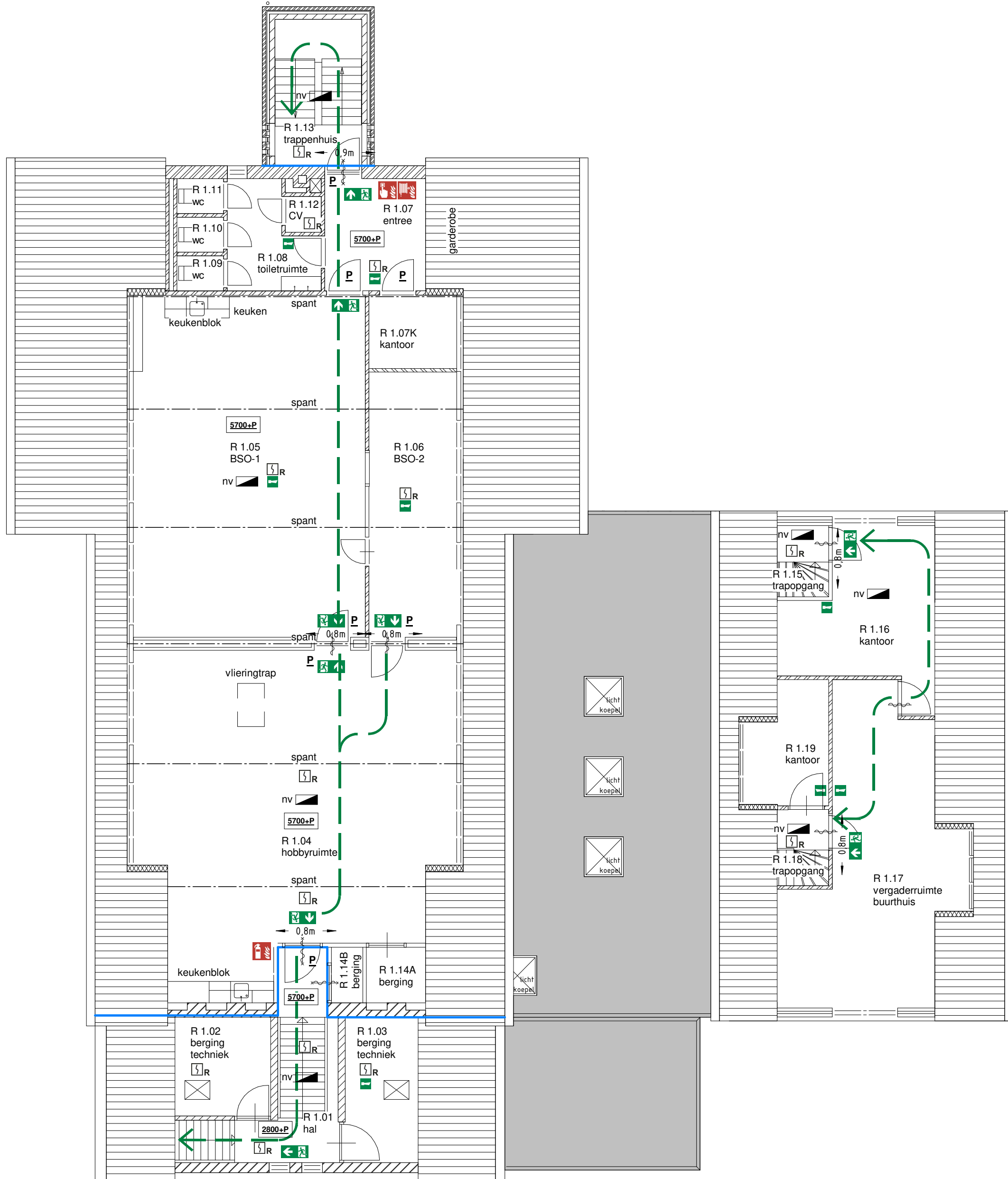
zolder 1:100
