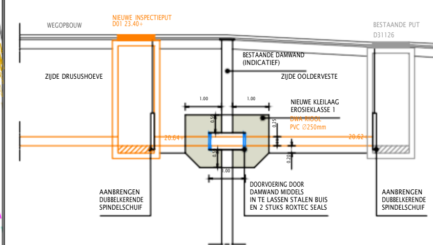
PRINCIPEDetail 1 SCHAAL 1:50
