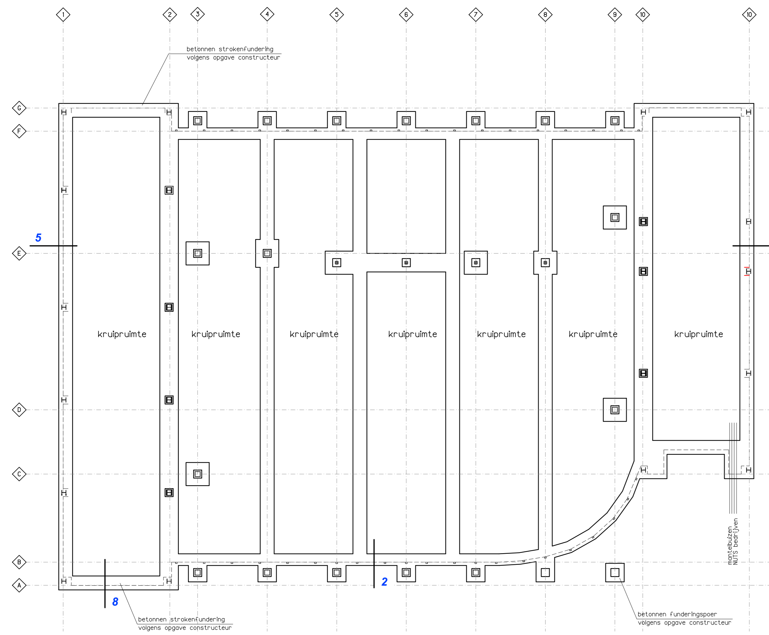
- FUNDERING / RIOLERINGPLAN -
