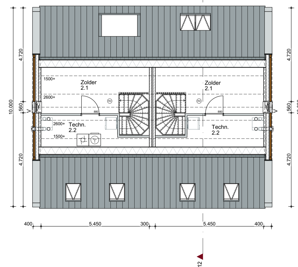
ZOLDER
