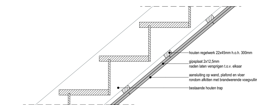
Principedetail trap 1:10
