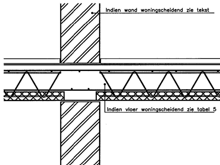
Detail II
