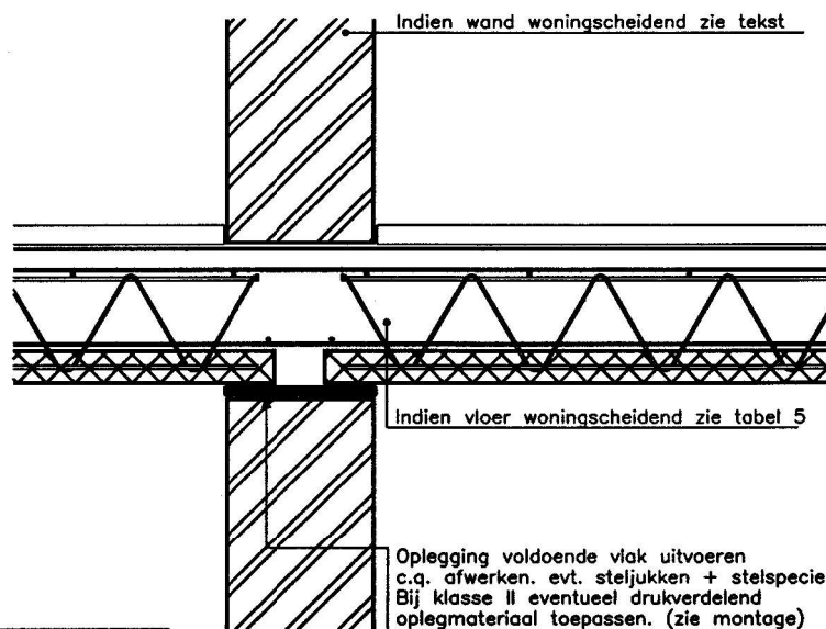
Detail IIa
