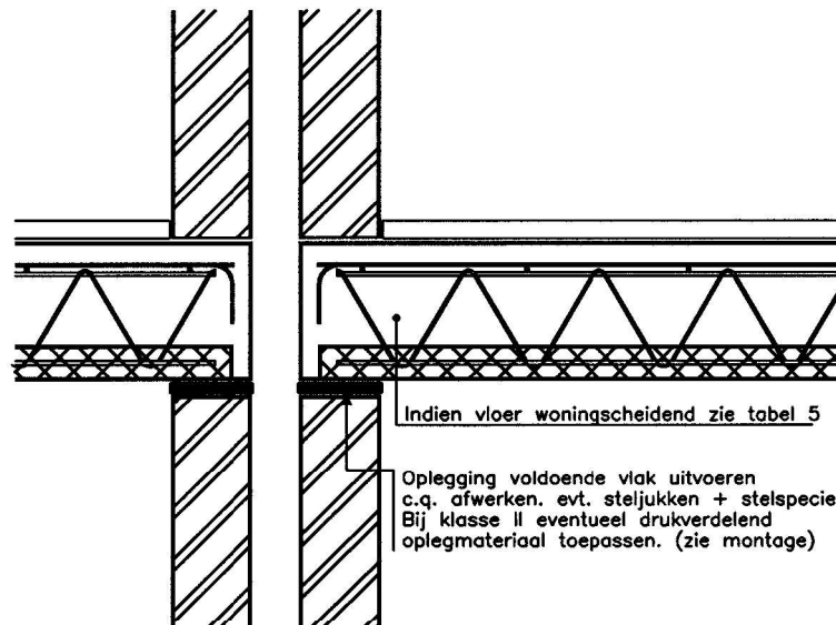
Detail Ia
