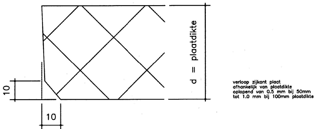
Randdetail
