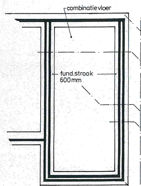
Fundering + Riolering
