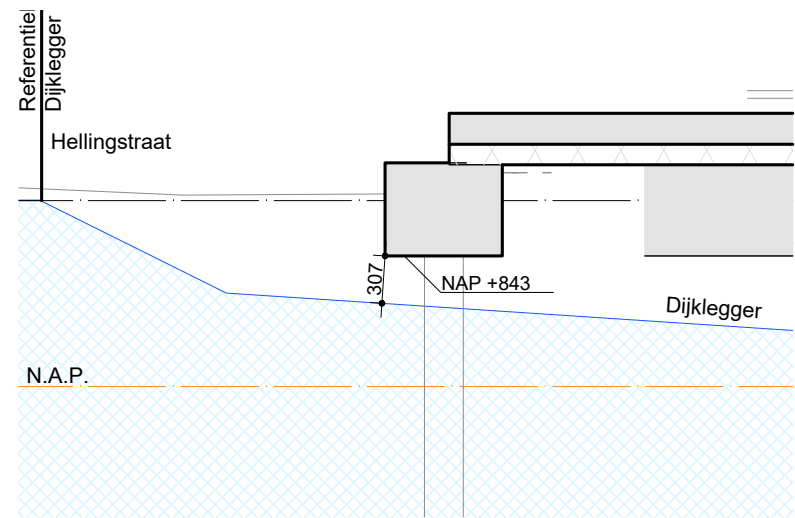
DETAIL 4 1:50
