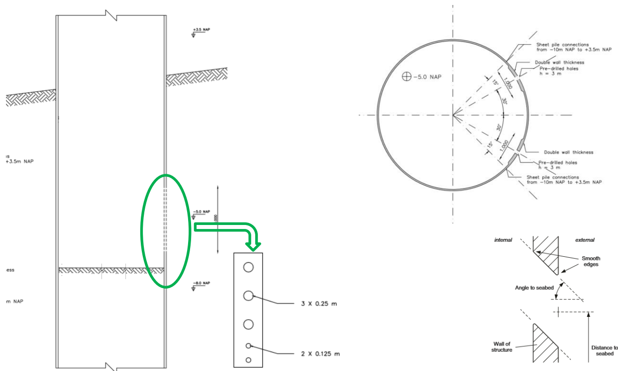
Figure 5-2: Grid connection provisions; DNVGL-RP-0360 fig 4-15 reference
