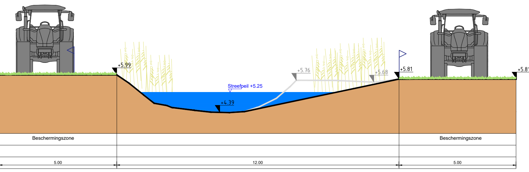
Profiel E-E'
